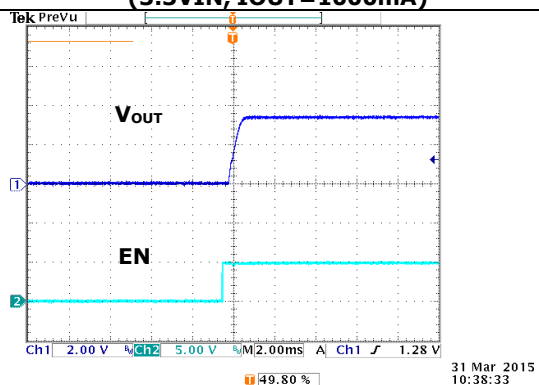
FIG.38 TURN-ON (3.3VIN, I_{OUT}=1000\text{mA} )
