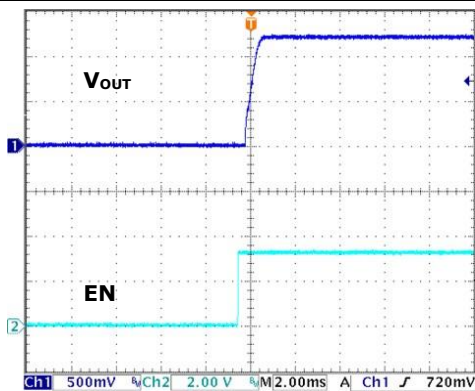
FIG.14 TURN-ON (3.3VIN, I_{OUT}=1000\text{mA} )
