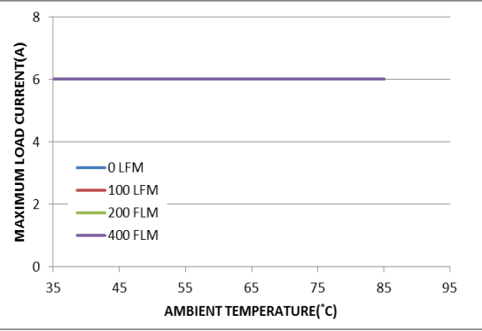
FIG.28 DE-RATING CURVE (VIN=12V, VOUT=3.3V)
