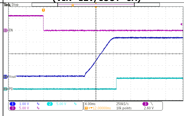
FIG.32 TURN-ON (VIN=12V, IOUT=6A)
