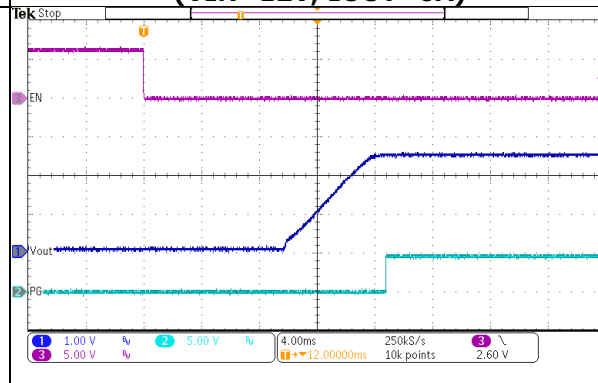
FIG.26 TURN-ON (VIN=12V, IOUT=6A)
