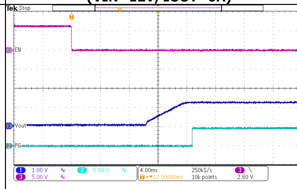
FIG.14 TURN-ON (VIN=12V, IOUT=6A)
