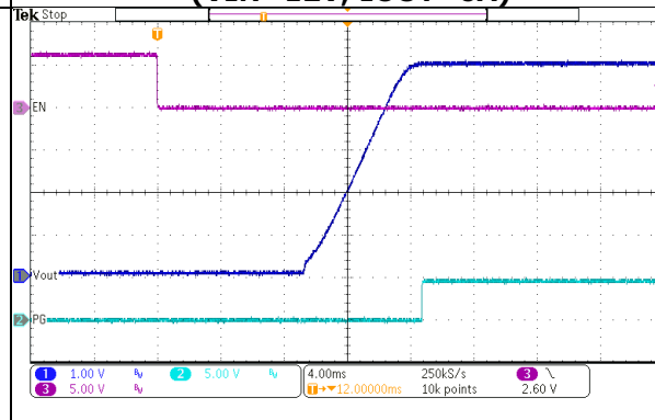
FIG.38 TURN-ON (VIN=12V, IOUT=6A)
