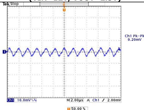
FIG.23 OUTPUT RIPPLE (VIN=12V, IOUT=0A)
