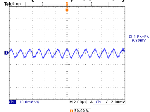
FIG.24 OUTPUT RIPPLE (VIN=12V, IOUT=6A)
