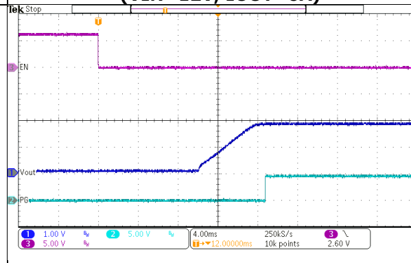
FIG.20 TURN-ON (VIN=12V, IOUT=6A)
