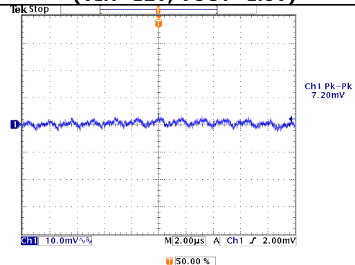
FIG.6 OUTPUT RIPPLE (VIN=12V, IOU=6A)
