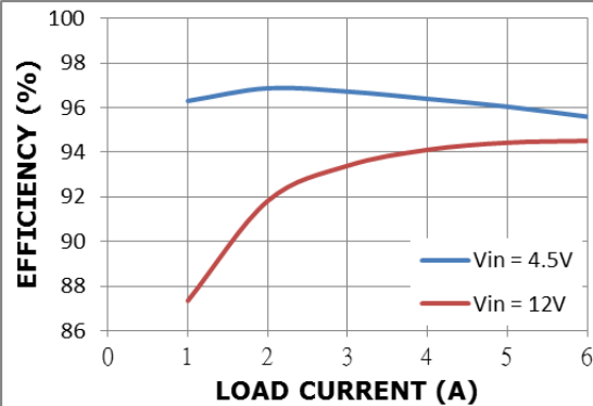
FIG.27 EFFICIENCY V.S. LOAD CURRENT (VIN=12V, VOUT=3.3V)
