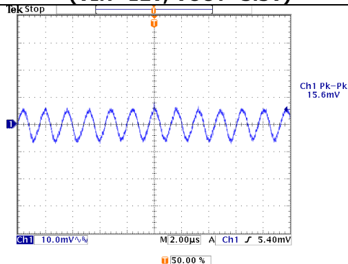
FIG.29 OUTPUT RIPPLE (VIN=12V, IOUT=0A)
