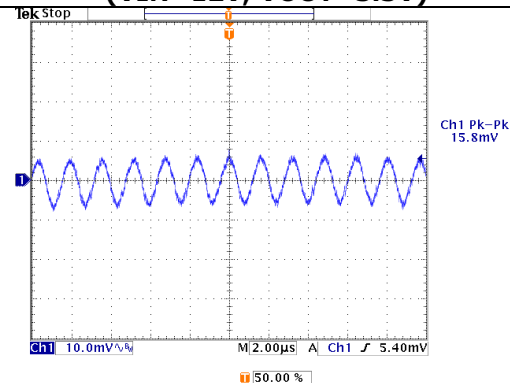
FIG.30 OUTPUT RIPPLE (VIN=12V, IOUT=6A)
