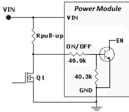
FIG.40 CIRCUIT FOR NEGATIVE ON/OFF LOGIC
