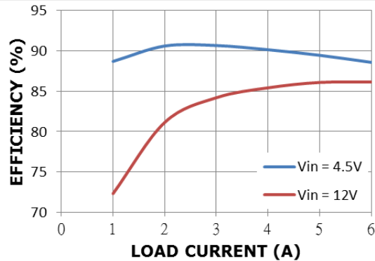
FIG.3 EFFICIENCY V.S. LOAD CURRENT (VIN=12V, VOUT=1.0V)
