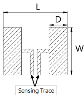
Recommended Dimensions of the Land Pad
